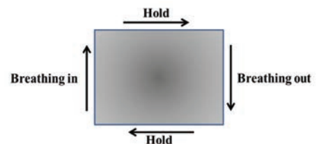
Fig. 9.17: Box-breathing
